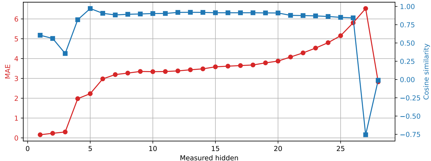
Qwen2.5-7B-Instruct | Prompt 1 Spared layer 14 | Unquantized vs hybrid
