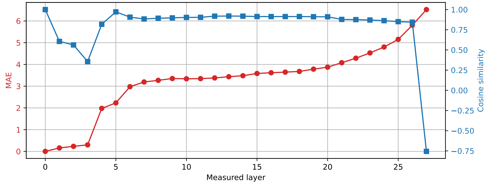
Qwen2.5-7B-Instruct | Prompt 1 Spared layer 14 | Hybrid vs unquantized
