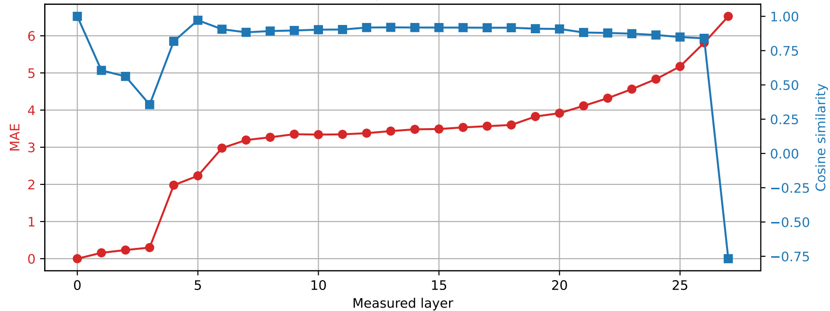
Qwen2.5-7B-Instruct | Prompt 1 Spared layer 18 | Hybrid vs unquantized
