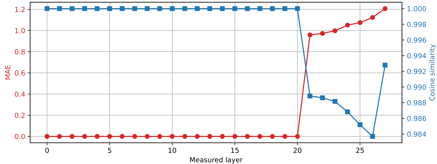
Qwen2.5-7B-Instruct | Prompt 1 Spared layer 20 | Hybrid vs quantized
