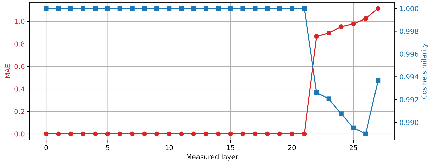
Qwen2.5-7B-Instruct | Prompt 1 Spared layer 21 | Hybrid vs quantized
