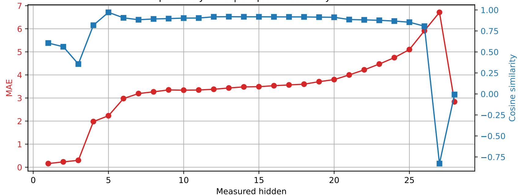
Qwen2.5-7B-Instruct | Prompt 1 Spared layer 25 | Unquantized vs hybrid
