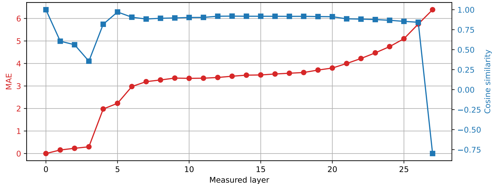
Qwen2.5-7B-Instruct | Prompt 1 Spared layer 26 | Hybrid vs unquantized
