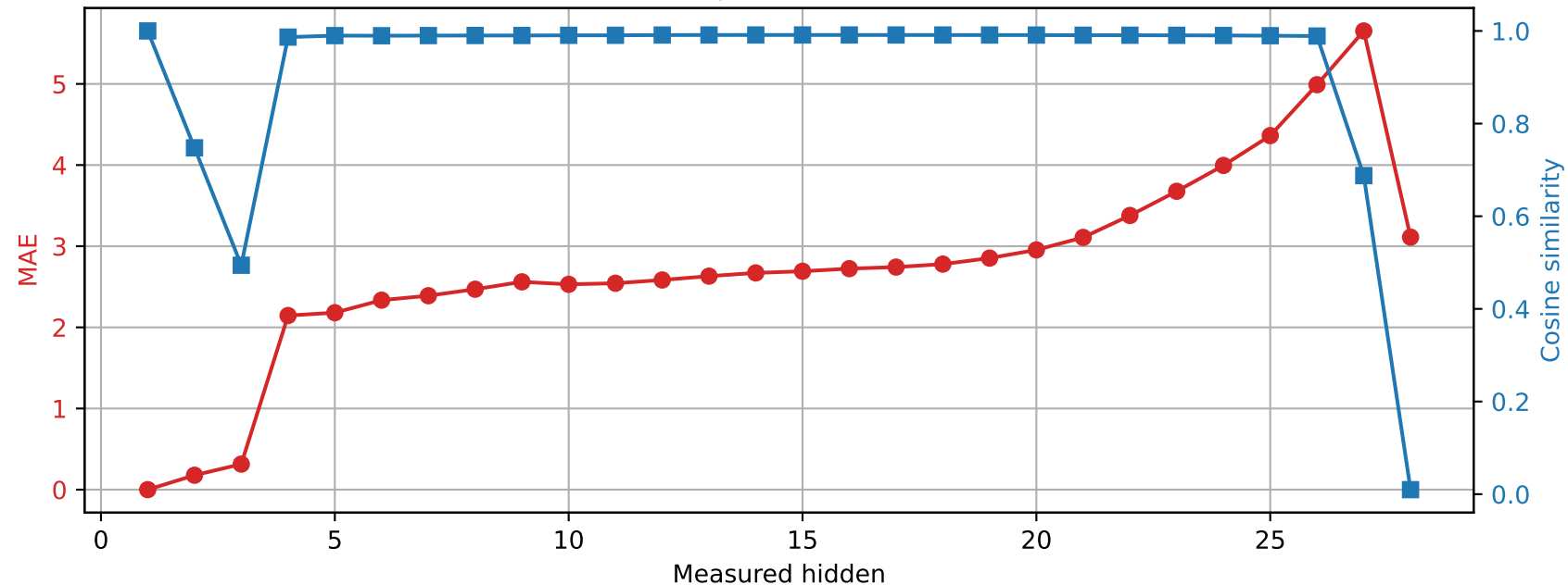
Qwen2.5-7B-Instruct | Prompt 2 Spared layer 0 | Unquantized vs hybrid
