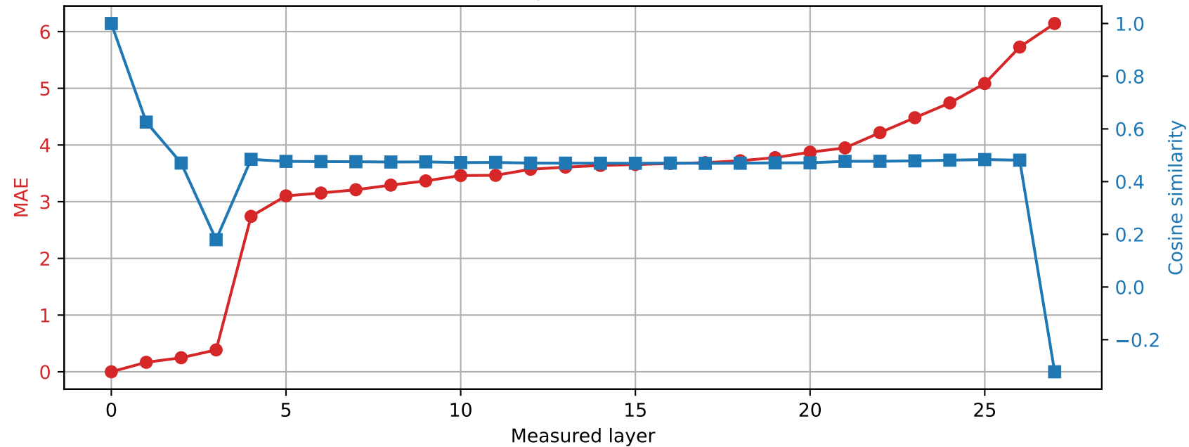
Qwen2.5-7B-Instruct | Prompt 2 Spared layer 9 | Hybrid vs unquantized
