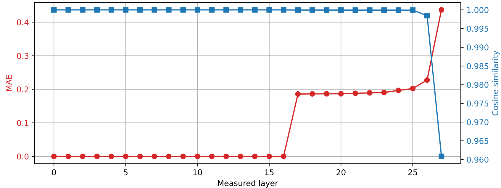
Qwen2.5-7B-Instruct | Prompt 2 Spared layer 16 | Hybrid vs quantized
