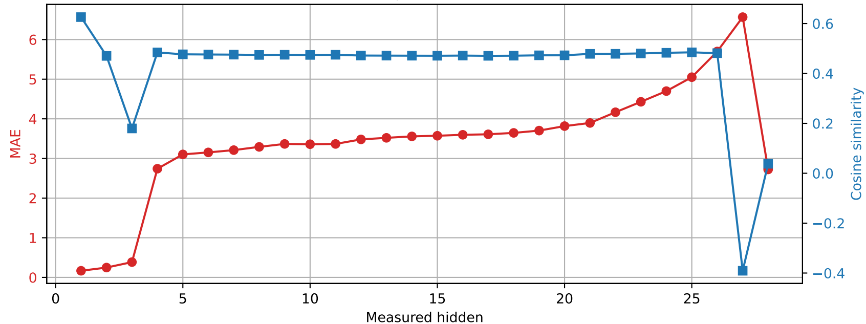
Qwen2.5-7B-Instruct | Prompt 2 Spared layer 19 | Unquantized vs hybrid
