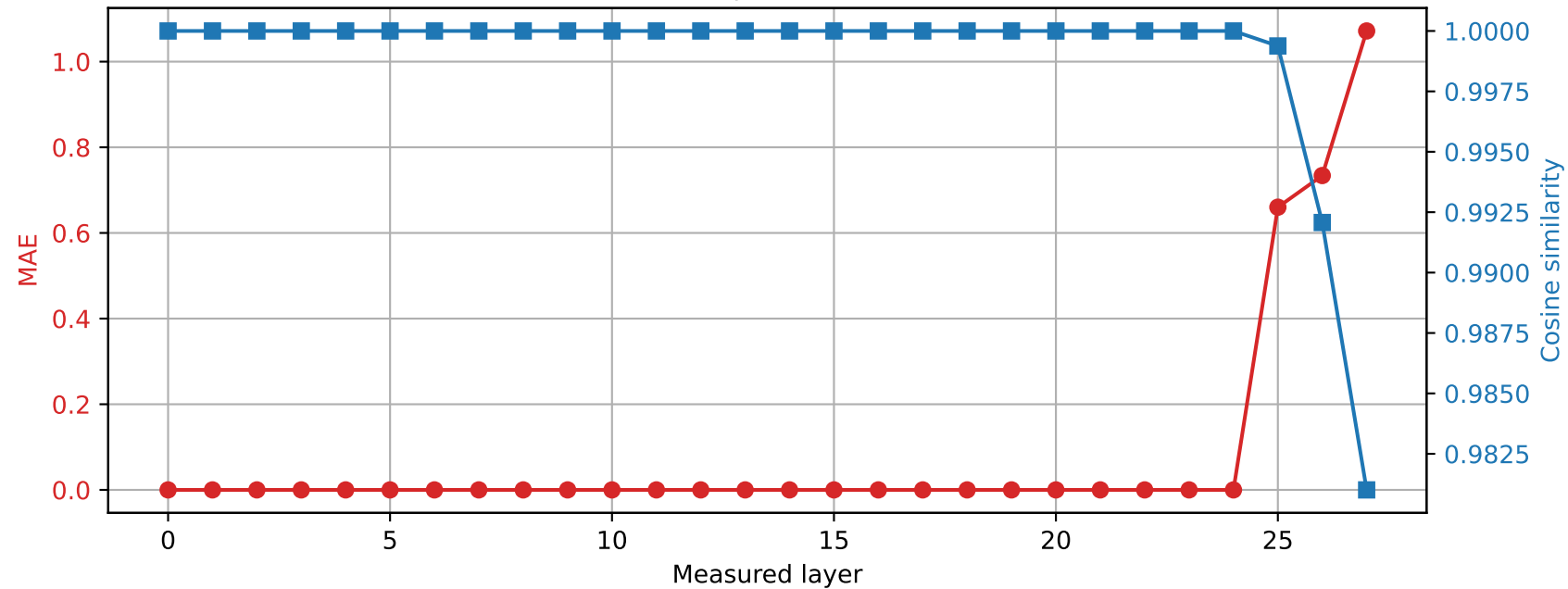
Qwen2.5-7B-Instruct | Prompt 2 Spared layer 24 | Hybrid vs quantized
