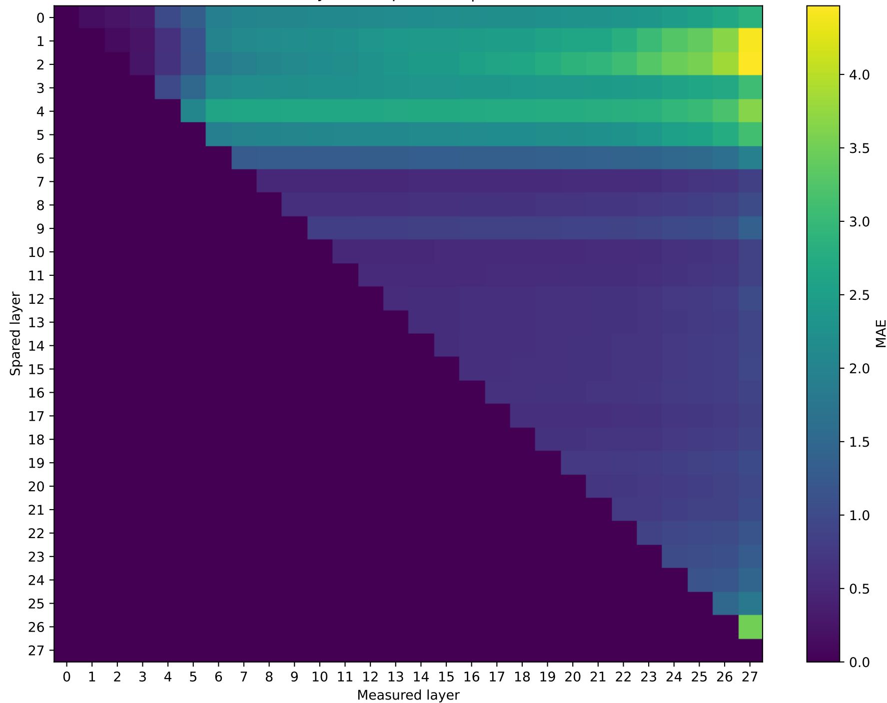
Qwen2.5-7B-Instruct | Prompt 3 Hybrid vs quantized | int4
