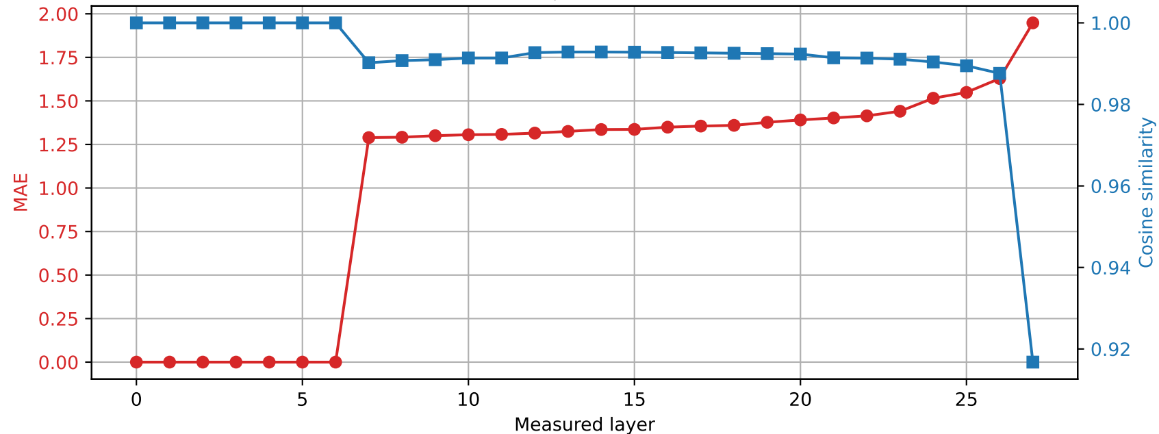
Qwen2.5-7B-Instruct | Prompt 3 Spared layer 6 | Hybrid vs quantized
