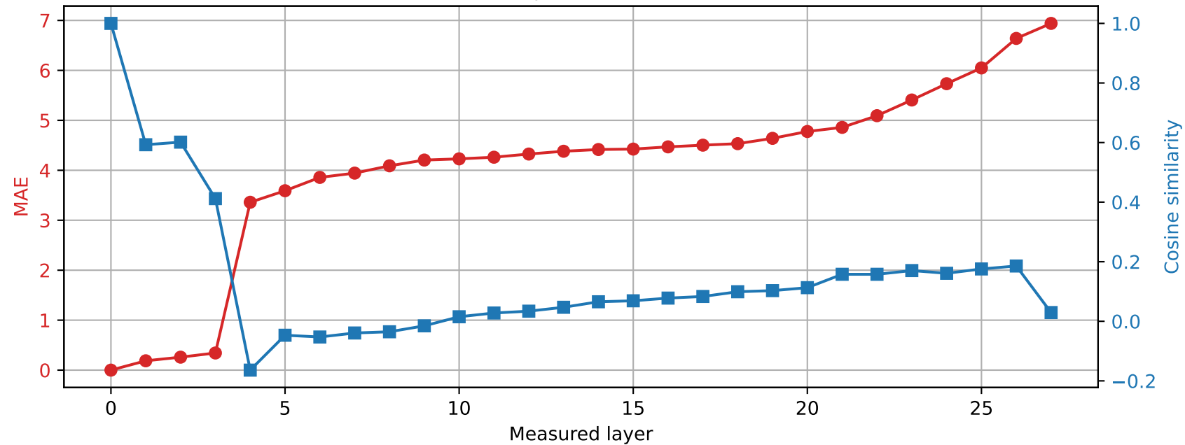
Qwen2.5-7B-Instruct | Prompt 4 Spared layer 1 | Hybrid vs unquantized
