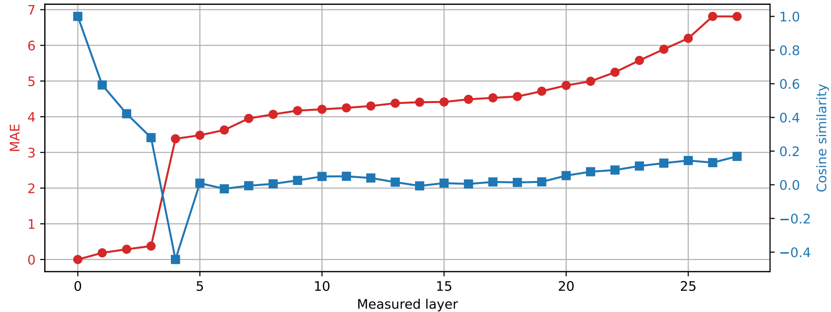
Qwen2.5-7B-Instruct | Prompt 4 Spared layer 6 | Hybrid vs unquantized
