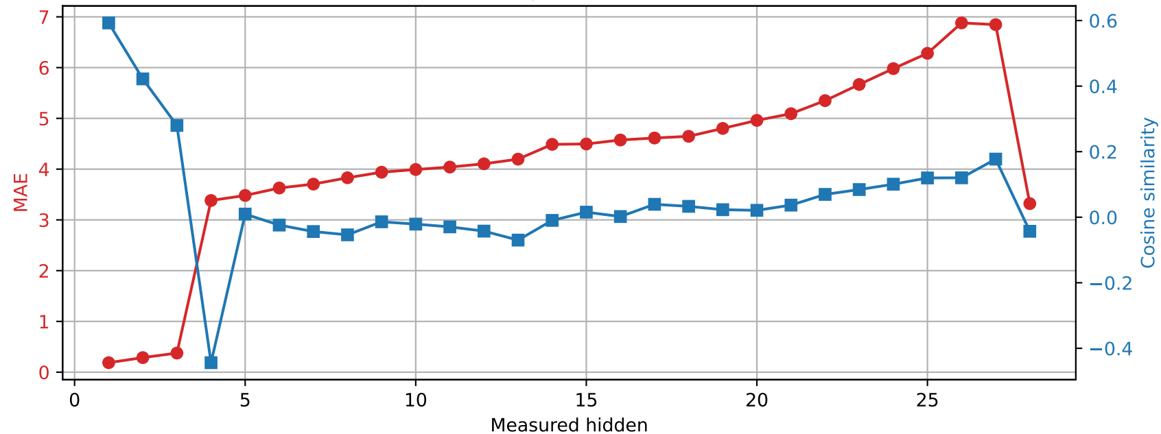
Qwen2.5-7B-Instruct | Prompt 4 Spared layer 13 | Unquantized vs hybrid
