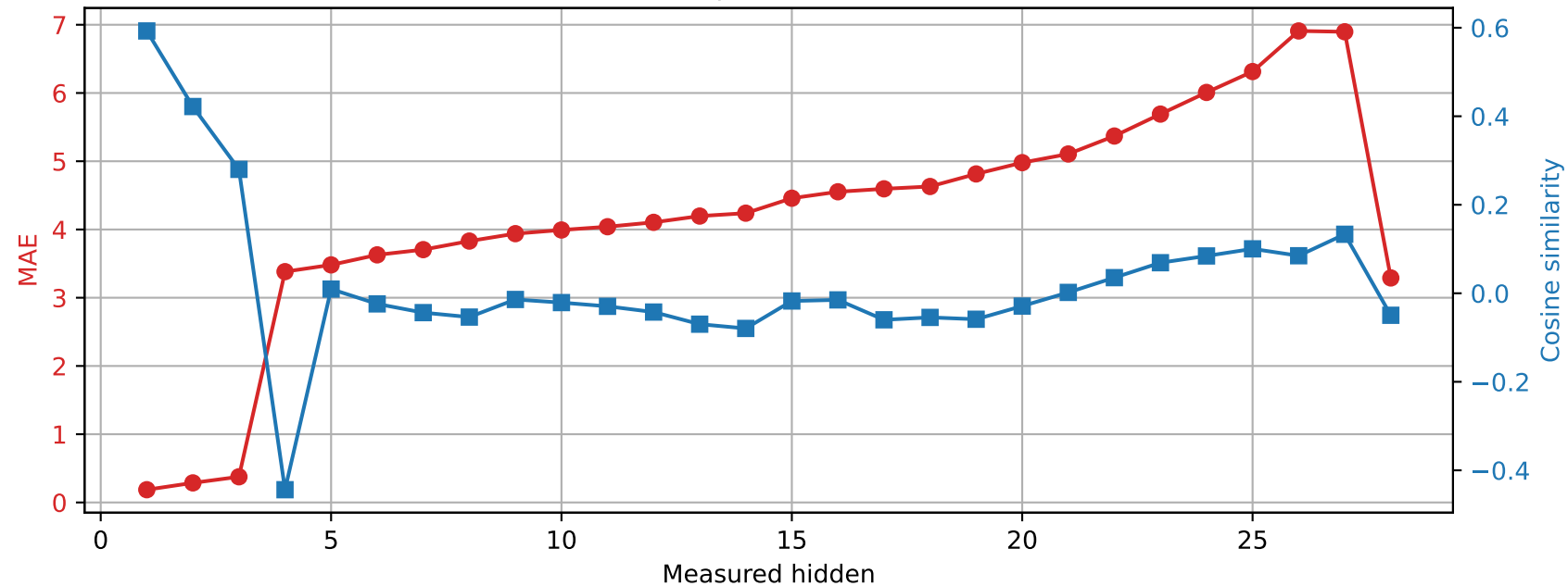
Qwen2.5-7B-Instruct | Prompt 4 Spared layer 14 | Unquantized vs hybrid
