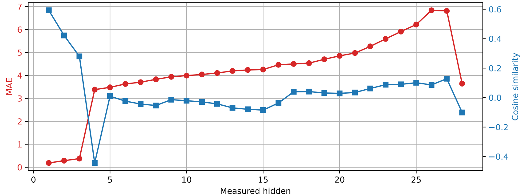
Qwen2.5-7B-Instruct | Prompt 4 Spared layer 15 | Unquantized vs hybrid
