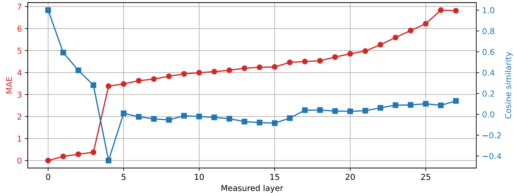
Qwen2.5-7B-Instruct | Prompt 4 Spared layer 15 | Hybrid vs unquantized
