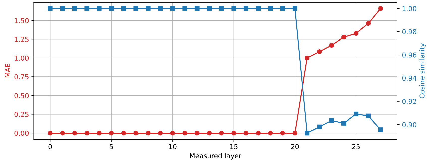
Qwen2.5-7B-Instruct | Prompt 4 Spared layer 20 | Hybrid vs quantized
