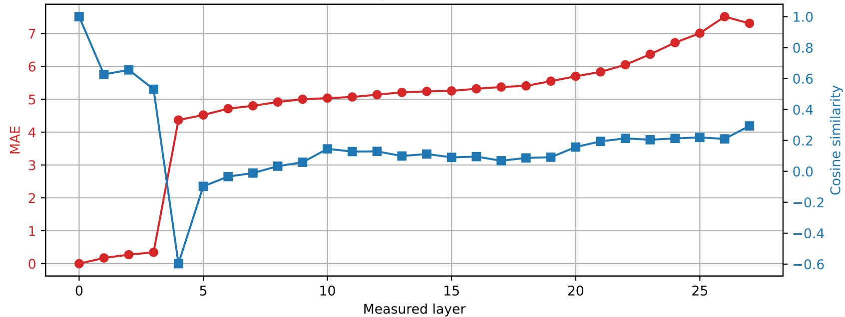
Qwen2.5-7B-Instruct | Prompt 0 Spared layer 1 | Hybrid vs unquantized
