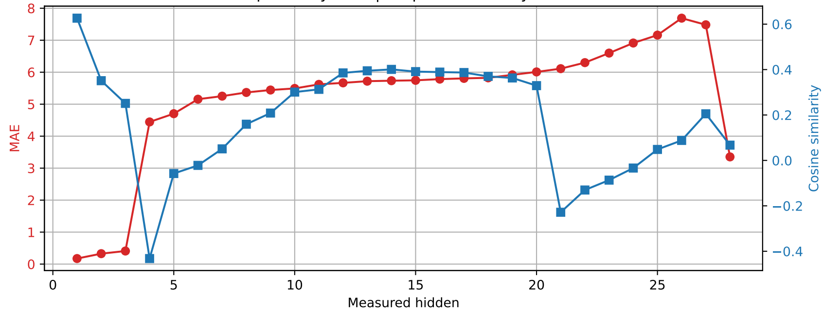
Qwen2.5-7B-Instruct | Prompt 0 Spared layer 10 | Unquantized vs hybrid
