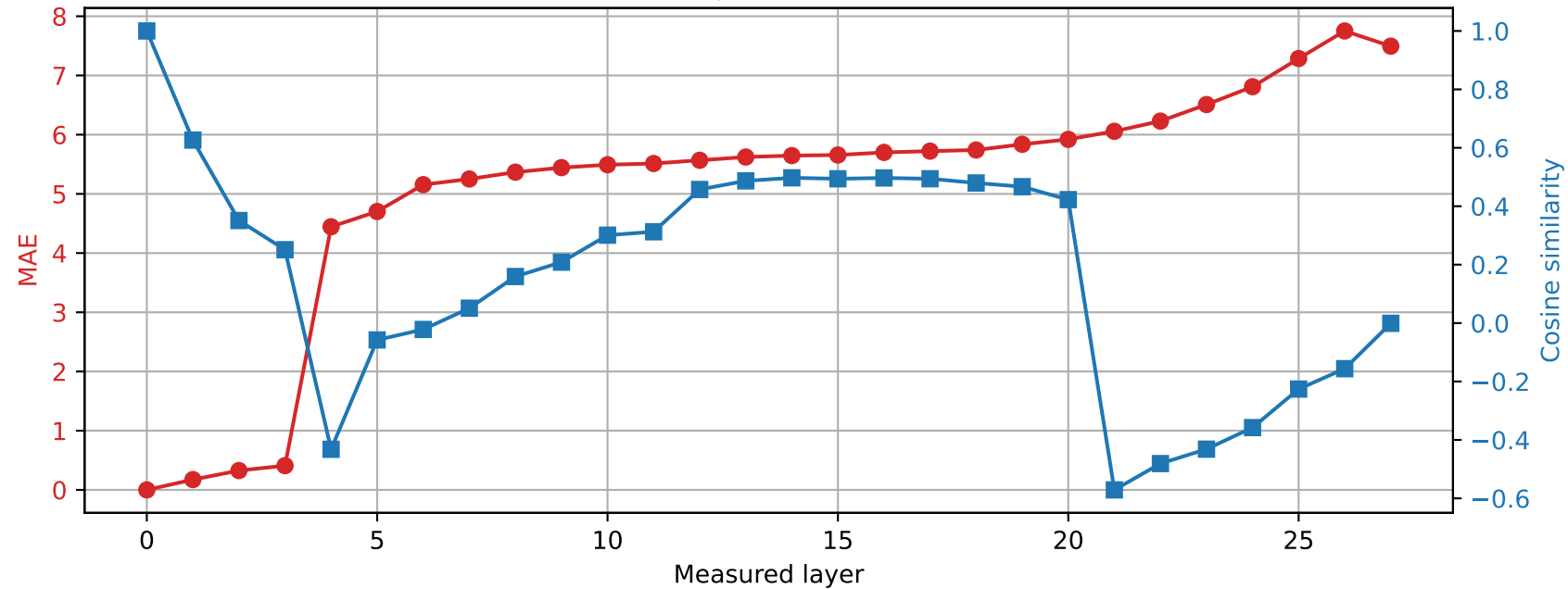
Qwen2.5-7B-Instruct | Prompt 0 Spared layer 24 | Hybrid vs unquantized
