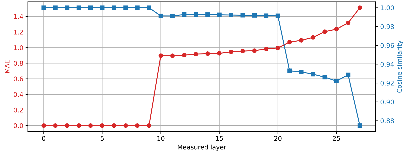
Qwen2.5-7B-Instruct | Prompt 1 Spared layer 9 | Hybrid vs quantized
