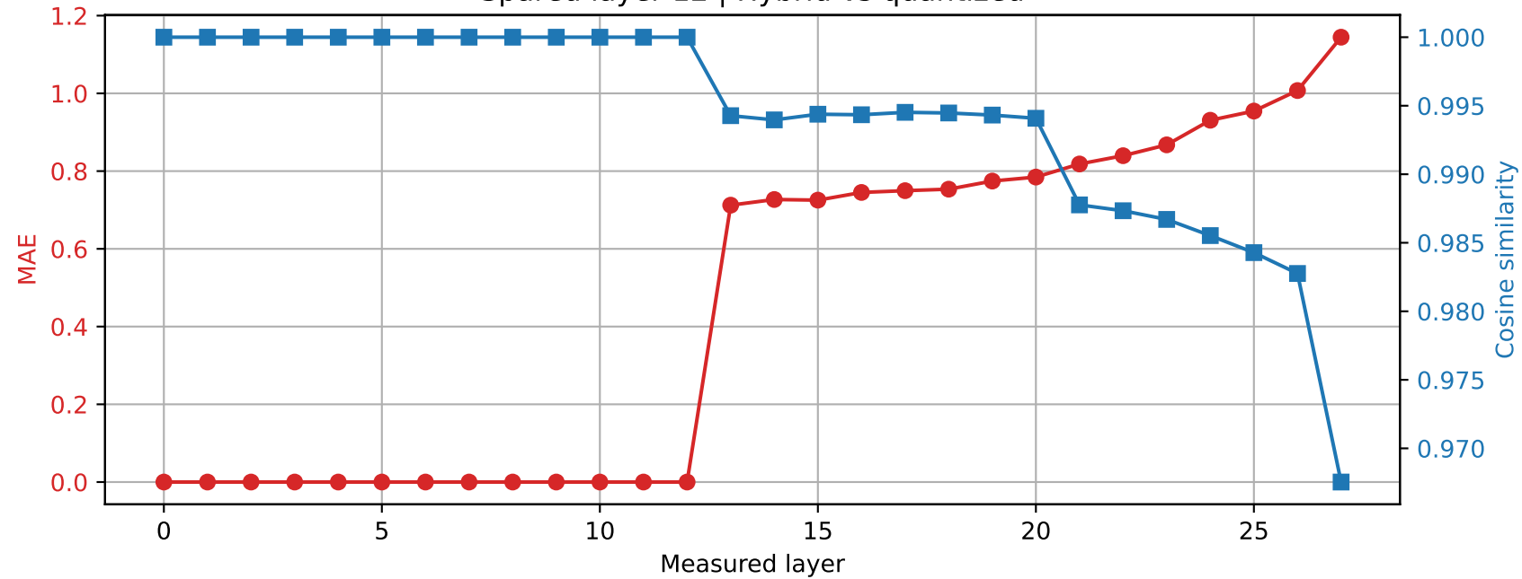
Qwen2.5-7B-Instruct | Prompt 1 Spared layer 12 | Hybrid vs quantized
