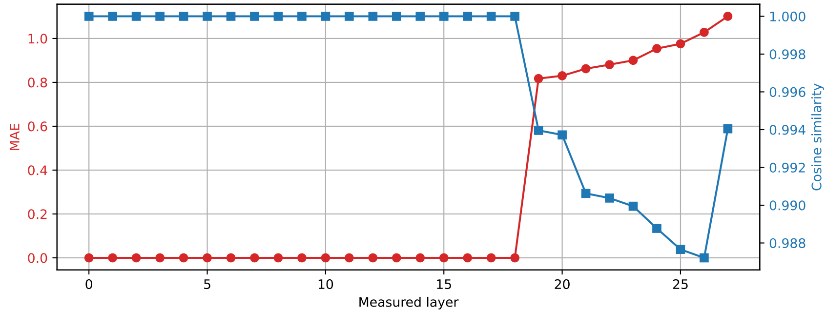
Qwen2.5-7B-Instruct | Prompt 1 Spared layer 18 | Hybrid vs quantized
