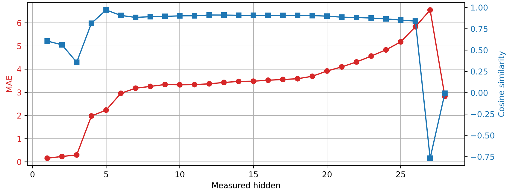
Qwen2.5-7B-Instruct | Prompt 1 Spared layer 19 | Unquantized vs hybrid
