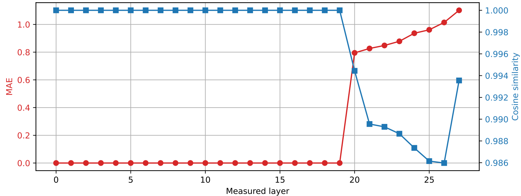
Qwen2.5-7B-Instruct | Prompt 1 Spared layer 19 | Hybrid vs quantized
