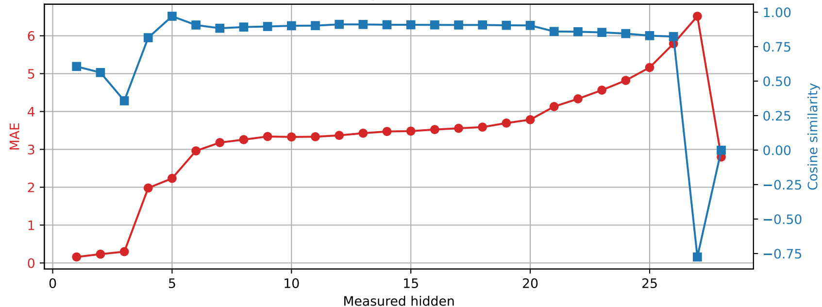
Qwen2.5-7B-Instruct | Prompt 1 Spared layer 20 | Unquantized vs hybrid
