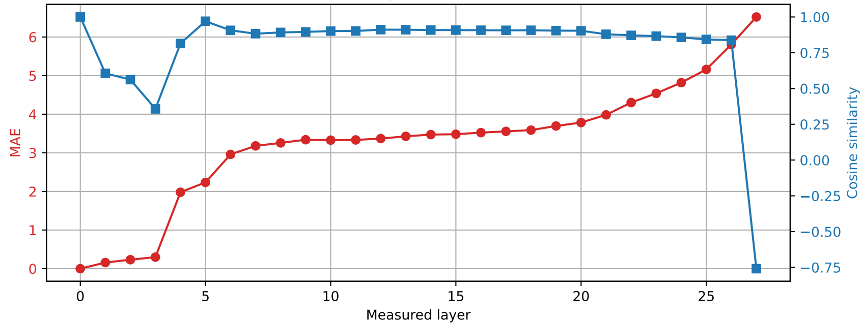
Qwen2.5-7B-Instruct | Prompt 1 Spared layer 21 | Hybrid vs unquantized
