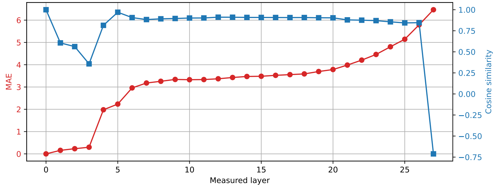
Qwen2.5-7B-Instruct | Prompt 1 Spared layer 23 | Hybrid vs unquantized
