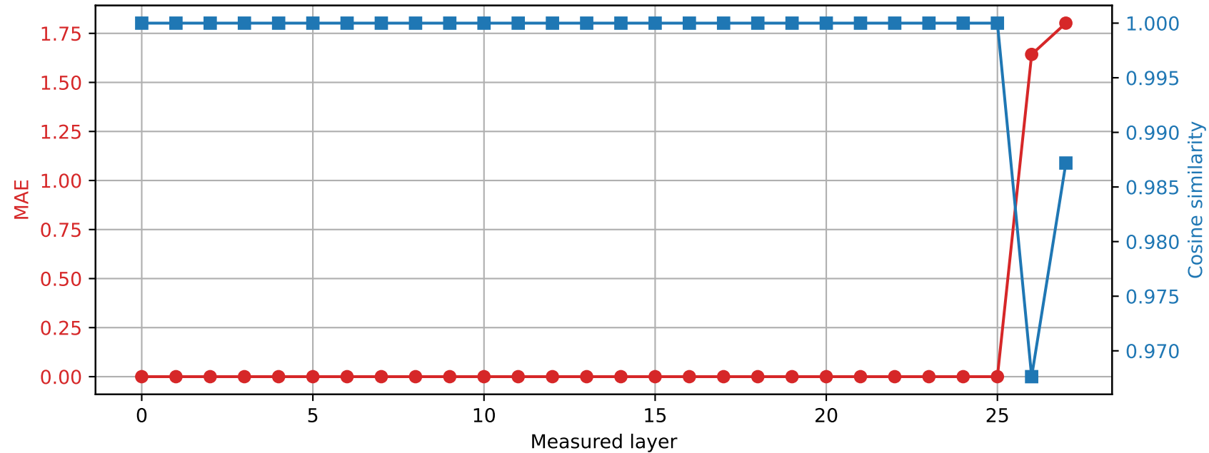
Qwen2.5-7B-Instruct | Prompt 1 Spared layer 25 | Hybrid vs quantized
