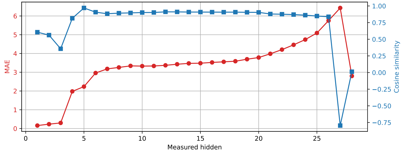
Qwen2.5-7B-Instruct | Prompt 1 Spared layer 26 | Unquantized vs hybrid
