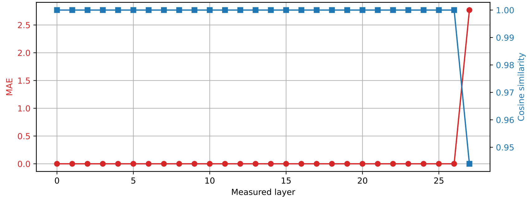
Qwen2.5-7B-Instruct | Prompt 1 Spared layer 26 | Hybrid vs quantized
