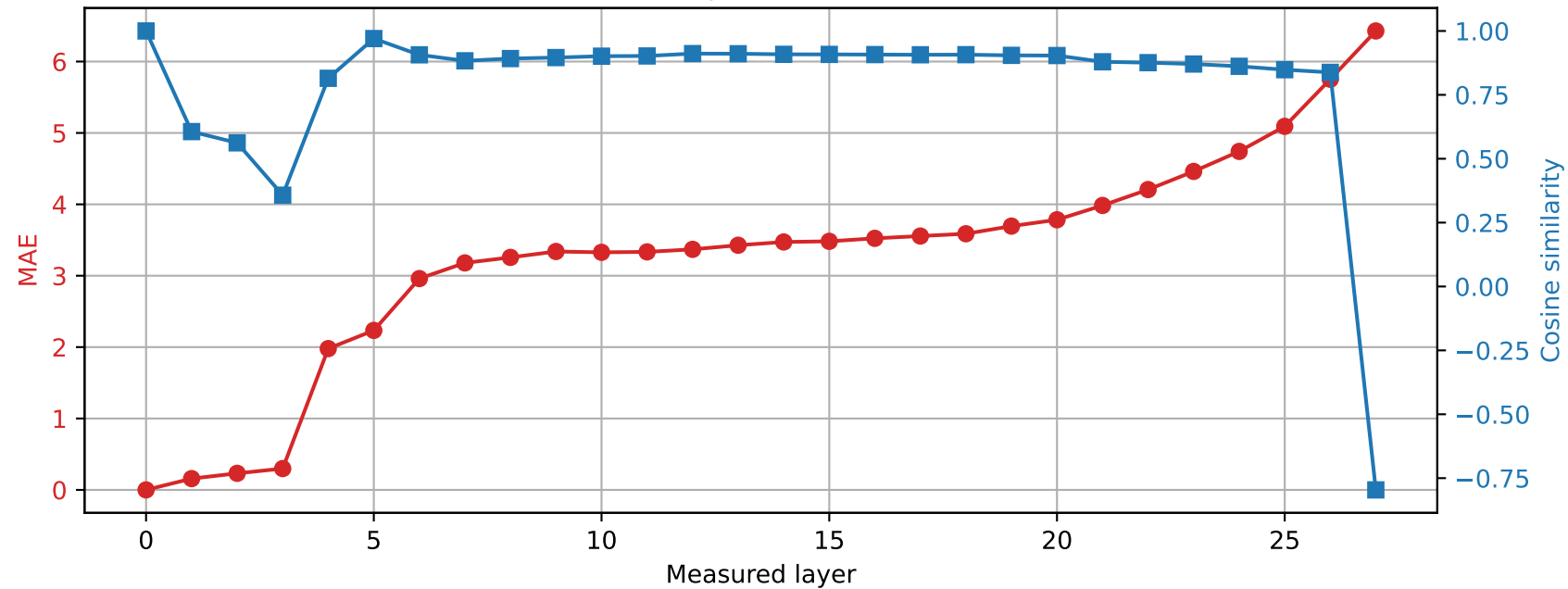
Qwen2.5-7B-Instruct | Prompt 1 Spared layer 26 | Hybrid vs unquantized
