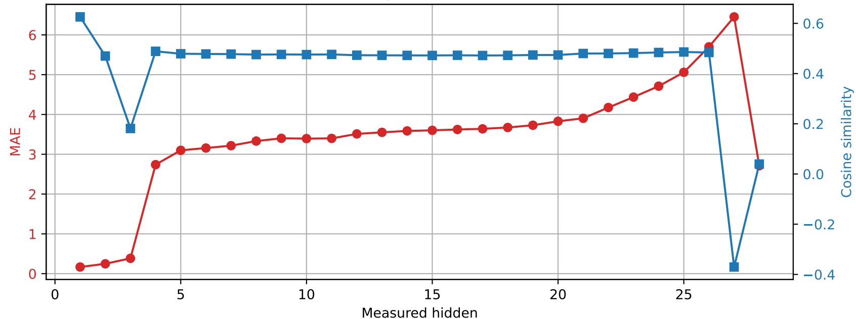
Qwen2.5-7B-Instruct | Prompt 2 Spared layer 7 | Unquantized vs hybrid
