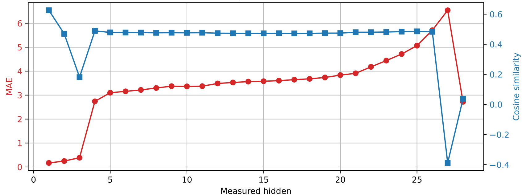
Qwen2.5-7B-Instruct | Prompt 2 Spared layer 16 | Unquantized vs hybrid
