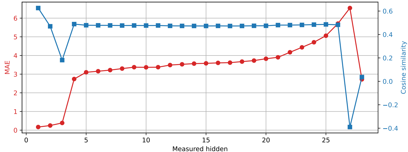
Qwen2.5-7B-Instruct | Prompt 2 Spared layer 17 | Unquantized vs hybrid
