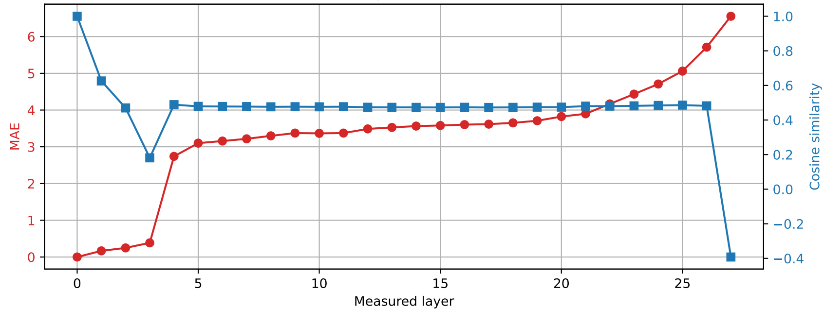
Qwen2.5-7B-Instruct | Prompt 2 Spared layer 19 | Hybrid vs unquantized
