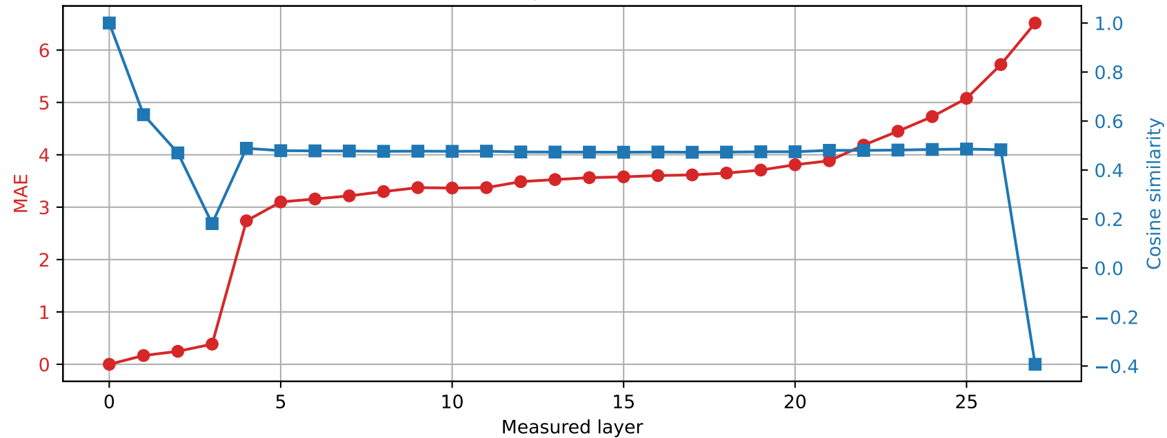
Qwen2.5-7B-Instruct | Prompt 2 Spared layer 21 | Hybrid vs unquantized
