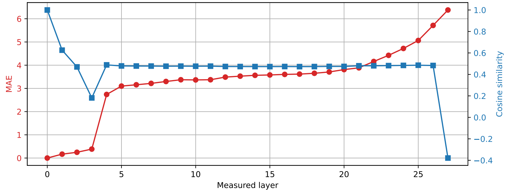
Qwen2.5-7B-Instruct | Prompt 2 Spared layer 23 | Hybrid vs unquantized
