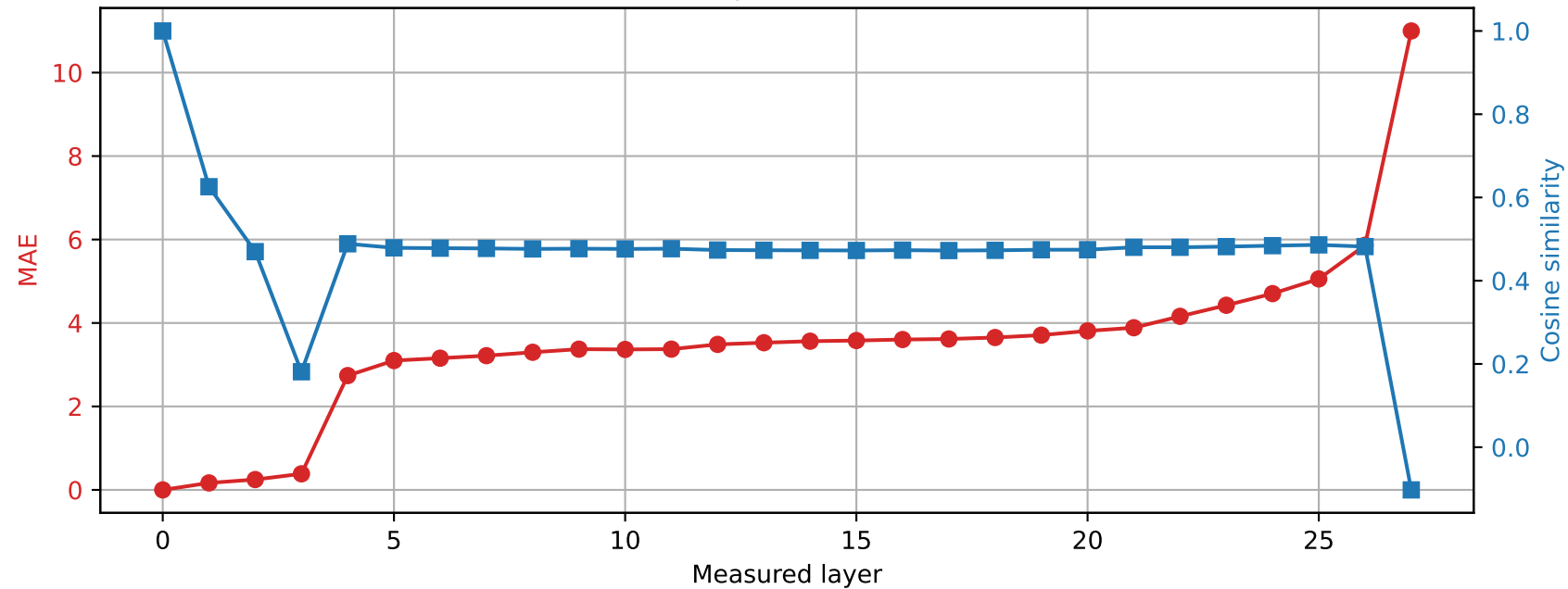
Qwen2.5-7B-Instruct | Prompt 2 Spared layer 25 | Hybrid vs unquantized
