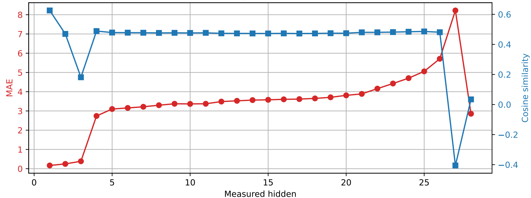
Qwen2.5-7B-Instruct | Prompt 2 Spared layer 26 | Unquantized vs hybrid
