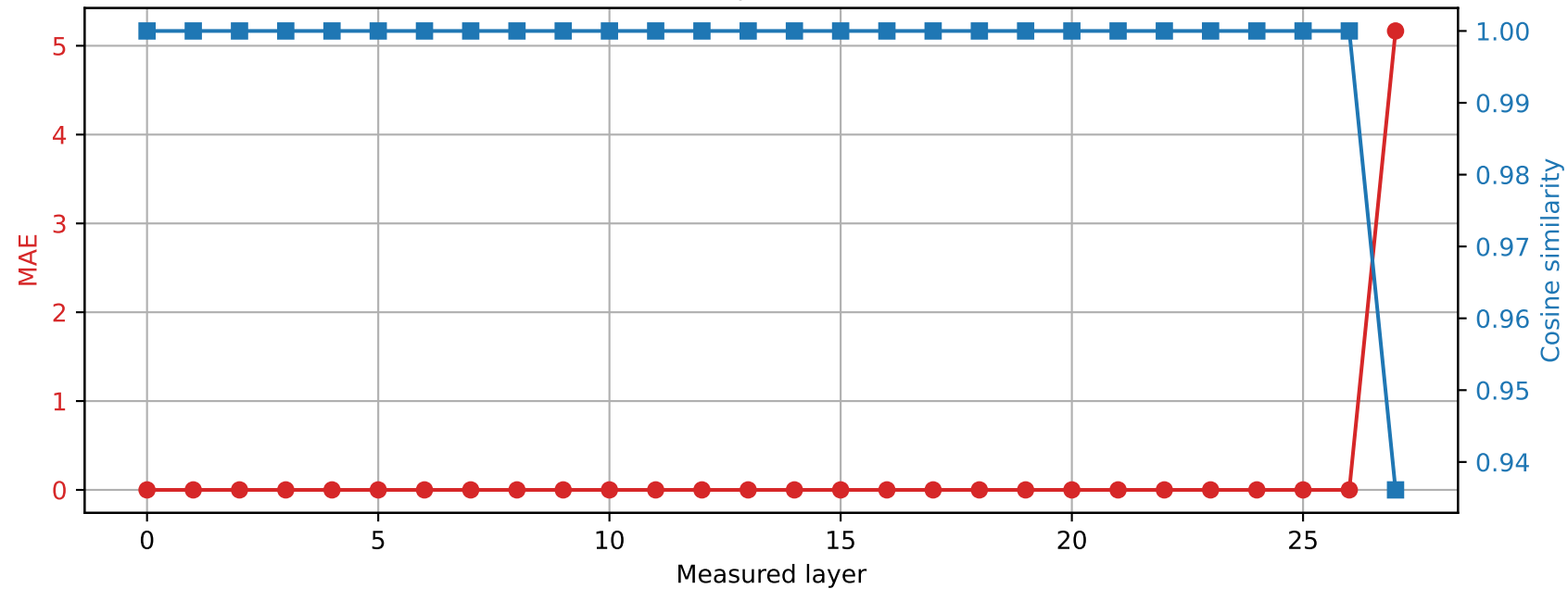
Qwen2.5-7B-Instruct | Prompt 2 Spared layer 26 | Hybrid vs quantized
