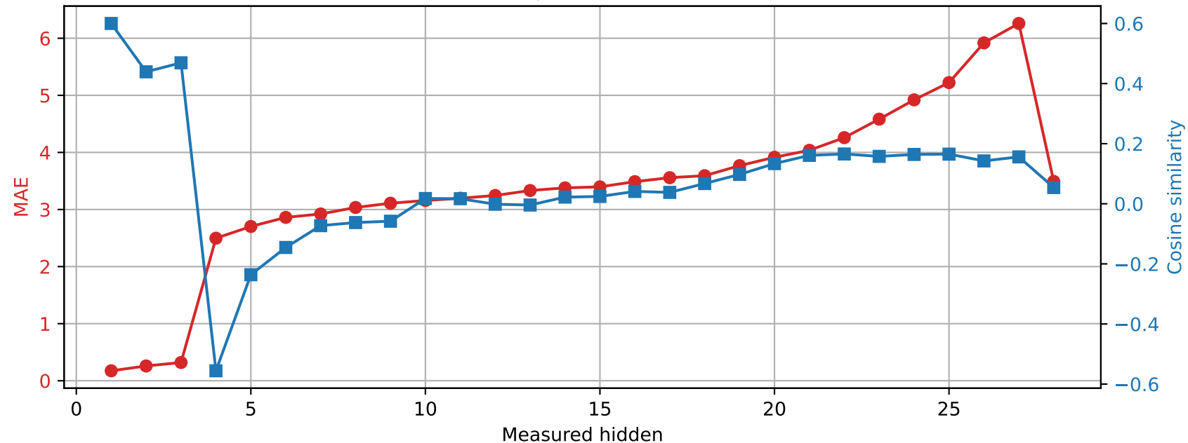
Qwen2.5-7B-Instruct | Prompt 3 Spared layer 2 | Unquantized vs hybrid
