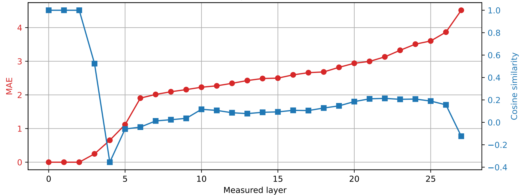
Qwen2.5-7B-Instruct | Prompt 3 Spared layer 2 | Hybrid vs quantized
