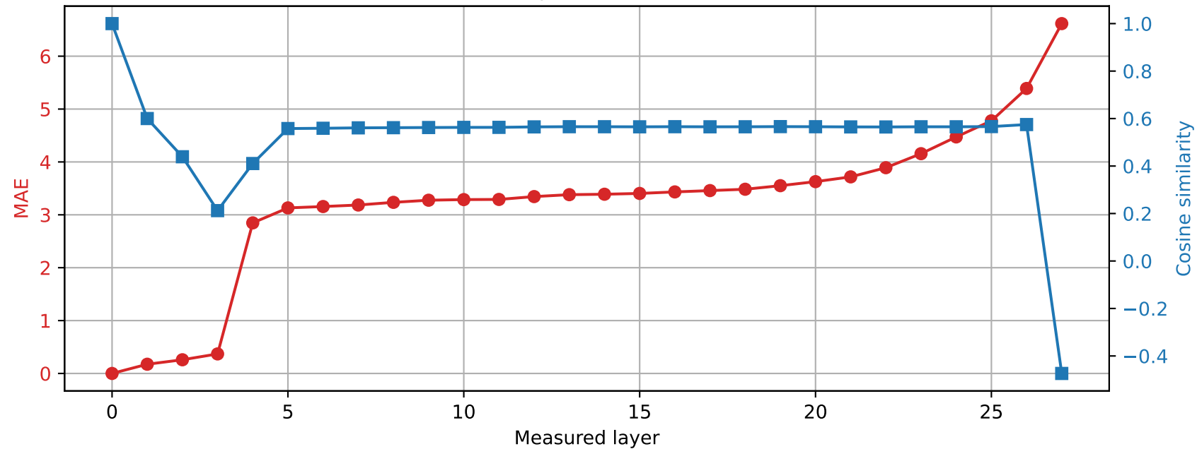
Qwen2.5-7B-Instruct | Prompt 3 Spared layer 3 | Hybrid vs unquantized
