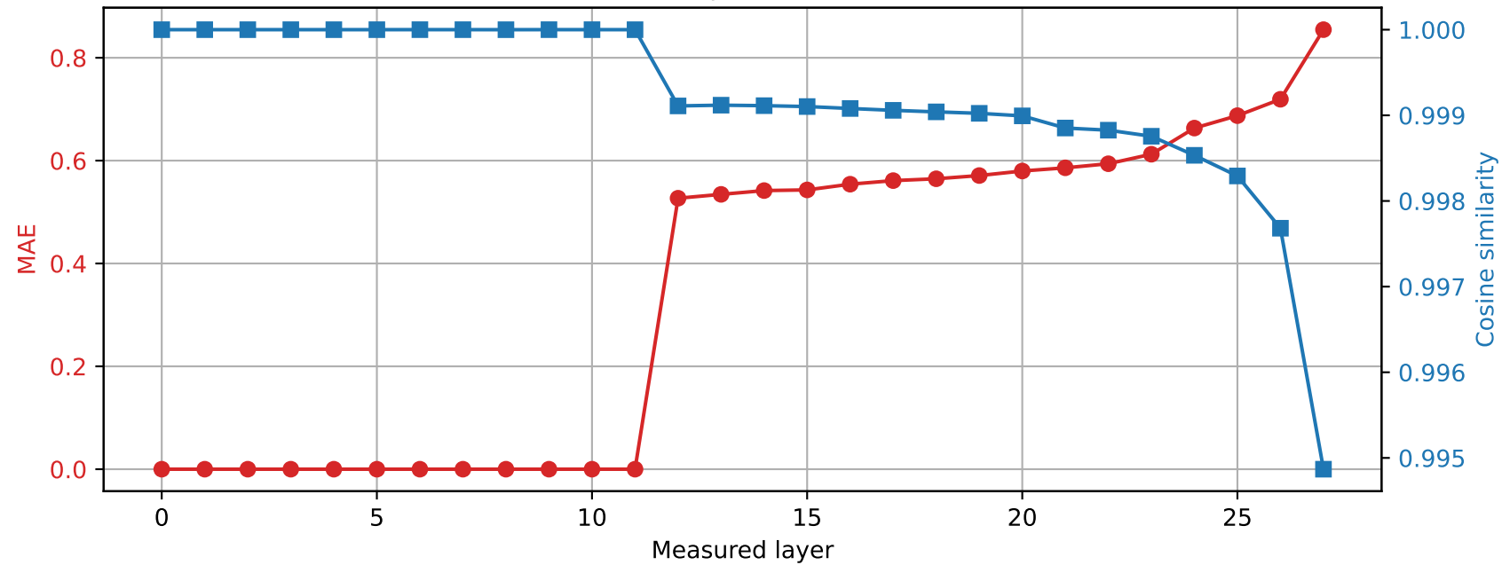
Qwen2.5-7B-Instruct | Prompt 3 Spared layer 11 | Hybrid vs quantized
