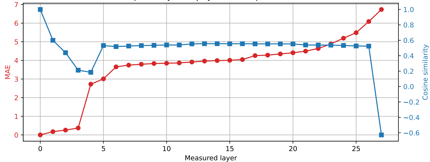
Qwen2.5-7B-Instruct | Prompt 3 Spared layer 16 | Hybrid vs unquantized
